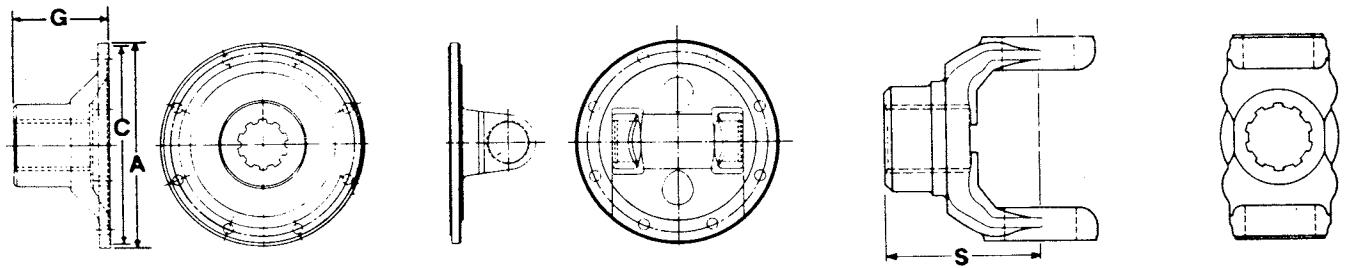
COMPANION FLANGE
